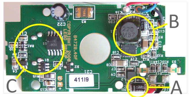
Figure 1: A copy of Philo's photograph of the printed circuit board (PCB) present in the LEGO LiPo rechargeable battery (#8878) ( http://www.brickshelf.com/cgi-bin/gallery.cgi?f=399263 )
