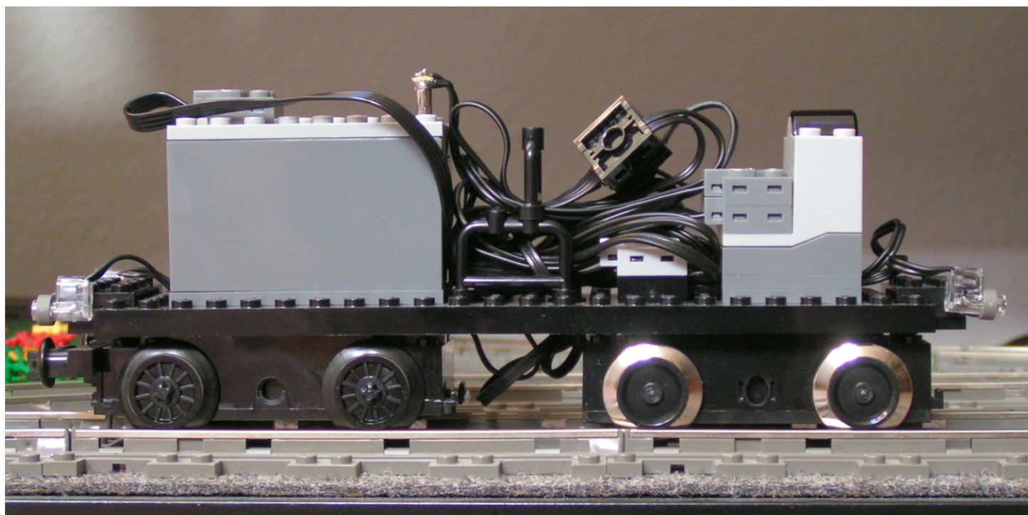
Figure 9: Compact PF/9 V "test bed" used for LiPo performance assessment. A modified 9 V train motor (power pickup and motor version, right) and an RC train motor are connected to output A of the PF receiver. Front and back LED lights are connected to output B. The receiver easily handles two train motors on one output.
