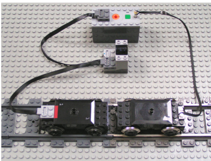
Figure 8: Principle of operation of combined PF/9 V trains. These are just two examples. Other combinations work as well. Left: "Power pickup only" version + RC motor. Right: "Power pickup and motor" version.
