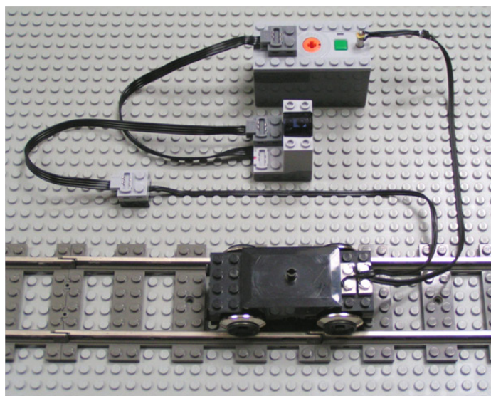
Figure 8: Principle of operation of combined PF/9 V trains. These are just two examples. Other combinations work as well. Left: "Power pickup only" version + RC motor. Right: "Power pickup and motor" version.
