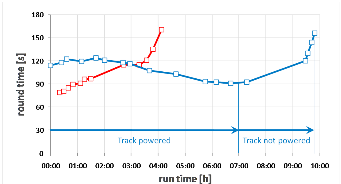
Figure 11: Round time measurements using the test set-up shown in figures 9 and 10.
