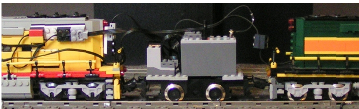
Figure 12: Heavier load test set-up. The PF test bed is coupled between both engines. It uses a “power pickup only” motor. The PF LiPo/receiver combination is powering everything, both 9V train motors (front truck of GP40, rear truck of GP38) and the GP40 head light.
