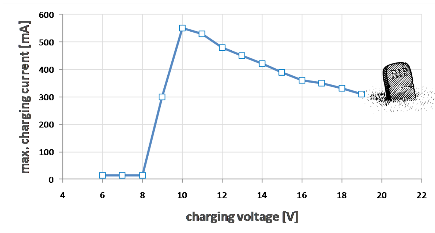
Figure 3: LiPo charging voltage vs. maximum “charging” current measurements. The maximum current was measured with a stalled PF XL motor present on the LiPo PF terminal set to full forward.
