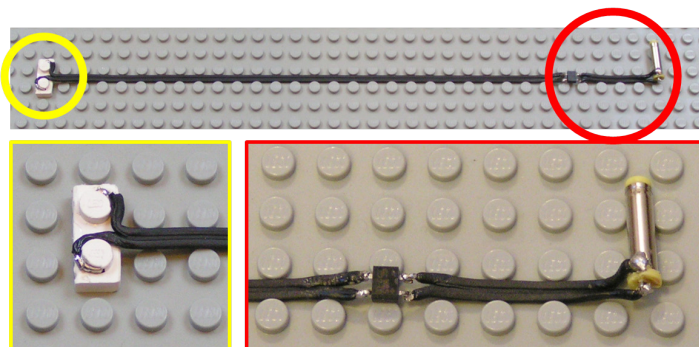
Figure 6: Photographs of the LiPo charging cable. Top: Complete assembly. Bottom: Close-ups of the soldered parts. Left: 1x2 terminal for the “power pickup and motor” version (see figure 4, top). Right: Bridge rectifier and DC plug.
