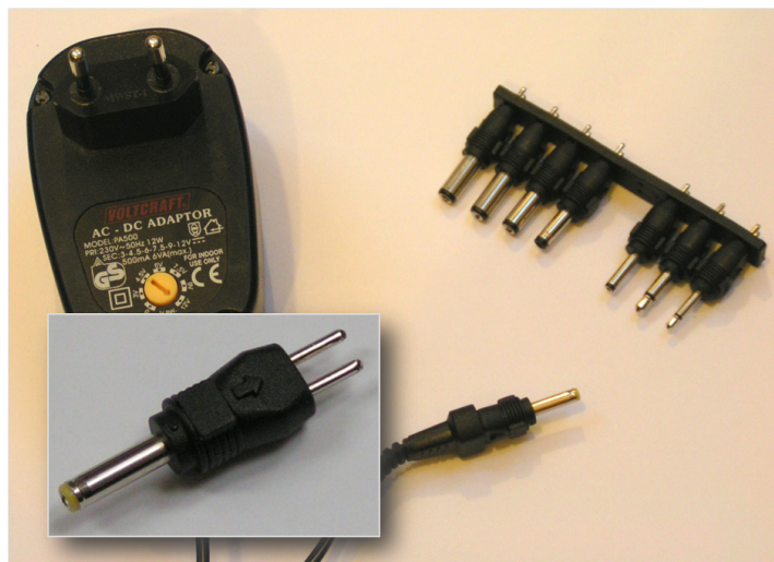
Figure 2: Photograph of a typical "wall wart" type power supply and the plug used for the charging experiments. Such power supplies often come with a variety of adaptor plugs. Insert: The 3.5 mm x 1.35 mm (x mm length, not important) plug works best with the LEGO PF LiPo.
