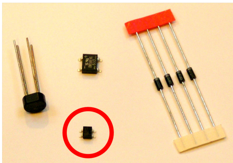
Figure 5: Left: Various types of bridge rectifiers; you could also use 4 discrete diodes shown on the right. I prefer the SMD type circled in red. The rated maximum current should be 1 A, just to be on the (very) safe side.
